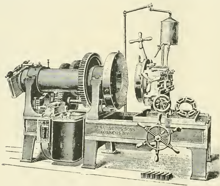
SAUNDERS' PIPE THREADING MACHINE.
